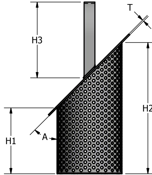
VIEW B-B SCALE 1 / 5
